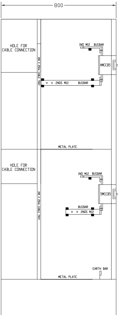
SECTION A
