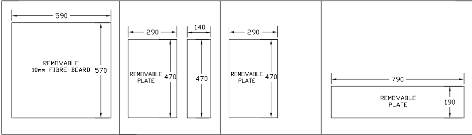
SECTION X (FLOOR MOUNTING/CABLE ENTRY DETAIL)
