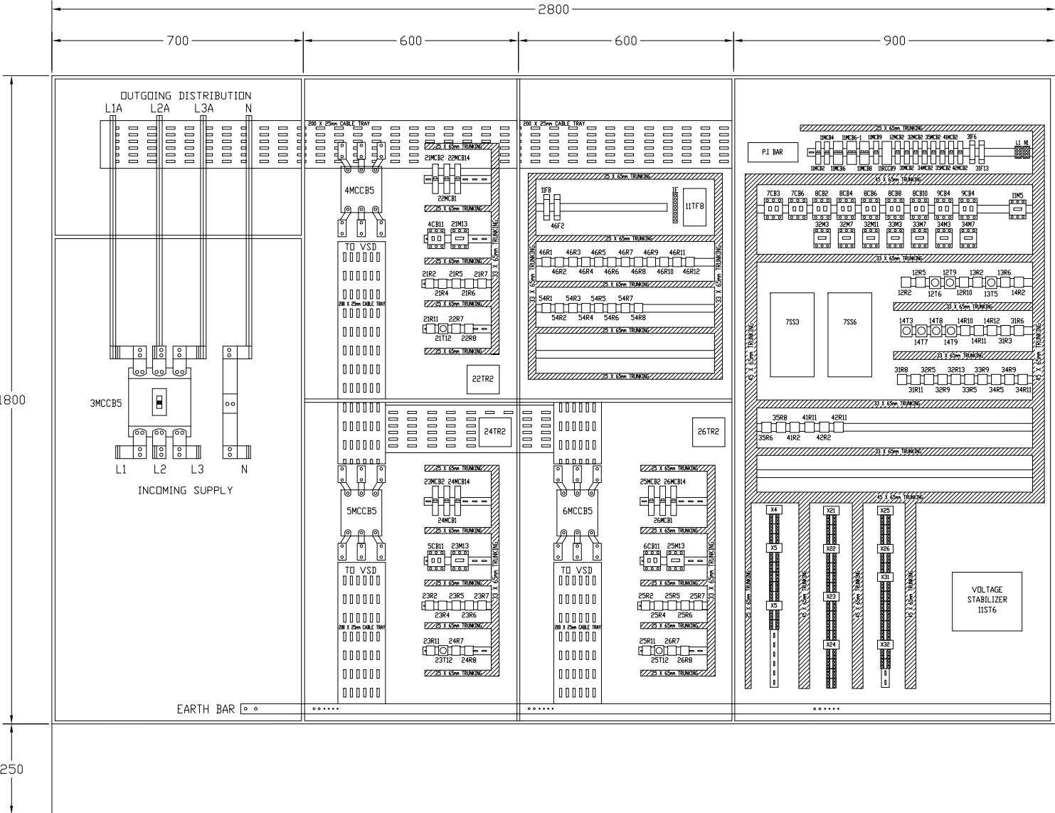
INTERNAL LAYOUT
